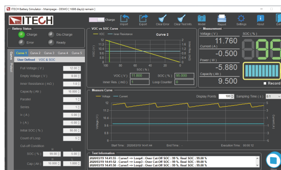
BSS2000 battery simulation software interface
